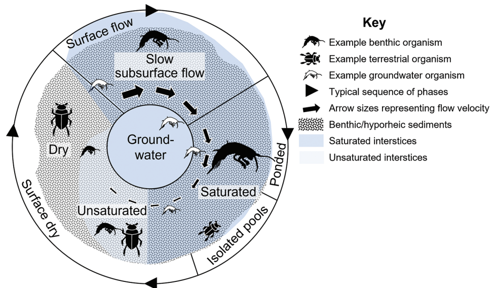
Figure 5. Biotic responses to temporal variability in hydrological conditions in the surface stream and benthic and subsurface sediments of nonperennial streams during a typical annual cycle. In a connected hyporheic zone, sediments can experience flowing phases, remain saturated during surface ponded and dry phases, gradually change from saturated to unsaturated then dry conditions after surface drying, then quickly rewet before surface flow resumes. Variability is less pronounced in the subsurface sediments compared with the surface stream and benthic sediments because flow velocities are slower during flowing phases, and interstices remain more humid after free water is lost. Benthic, groundwater, and terrestrial organisms respond to changing conditions differently. Variation in symbol size is proportional to expected densities of the represented organism.
